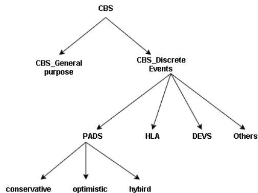
Figure 5: Illustration of CBS types and the focus branches addressed in this paper.
