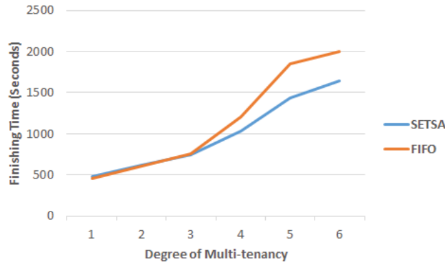
Figure 3: Performance of ASETS compared with FIFO scheduling in a private cloud.
