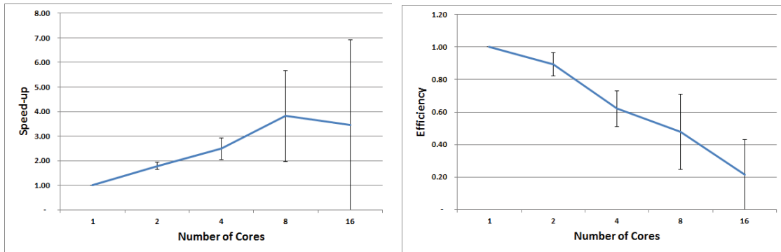
Figure 1: Speed-up (a) and Efficiency (b) of a Matrix Multiplication benchmark on Amazon EC2 instance.
